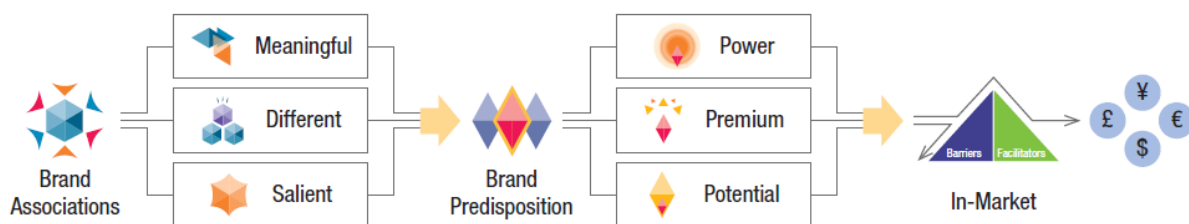
Figure 9.2 Brand Dynamics
