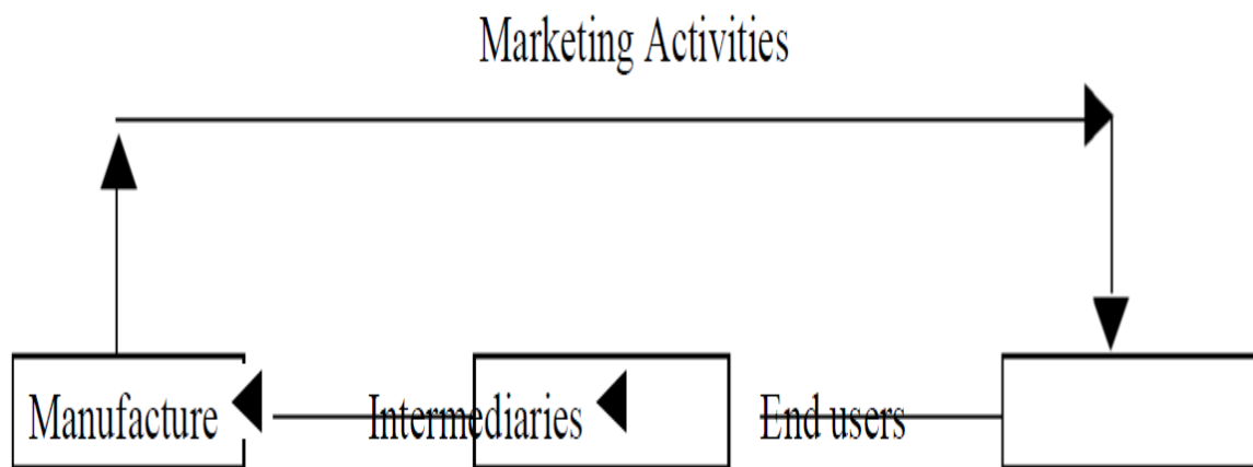
Figure 7.1 Pull Strategy
