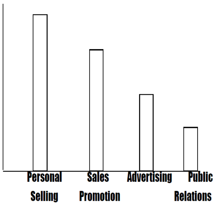
Figure 7.3 Industrial Goods
